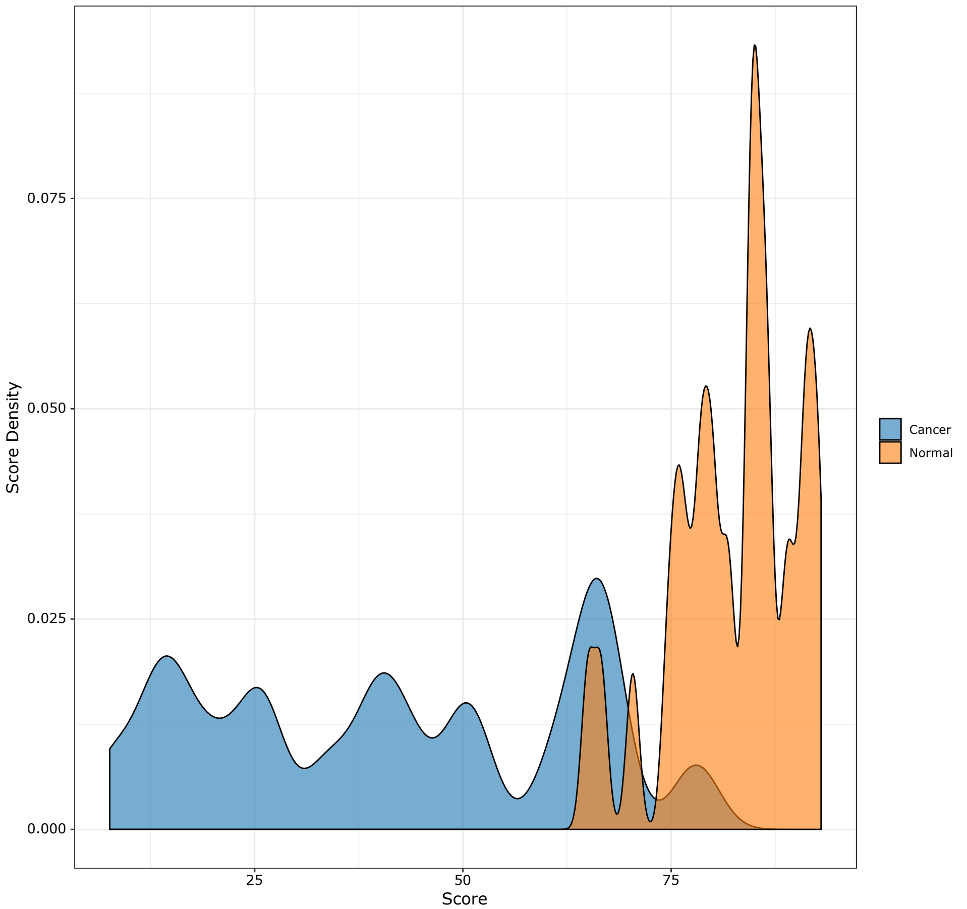
Score distribution
